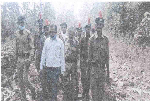
Forest tracking in Katepurna forest
